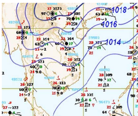
Figure 1: Weather map for 13 th October 2015
