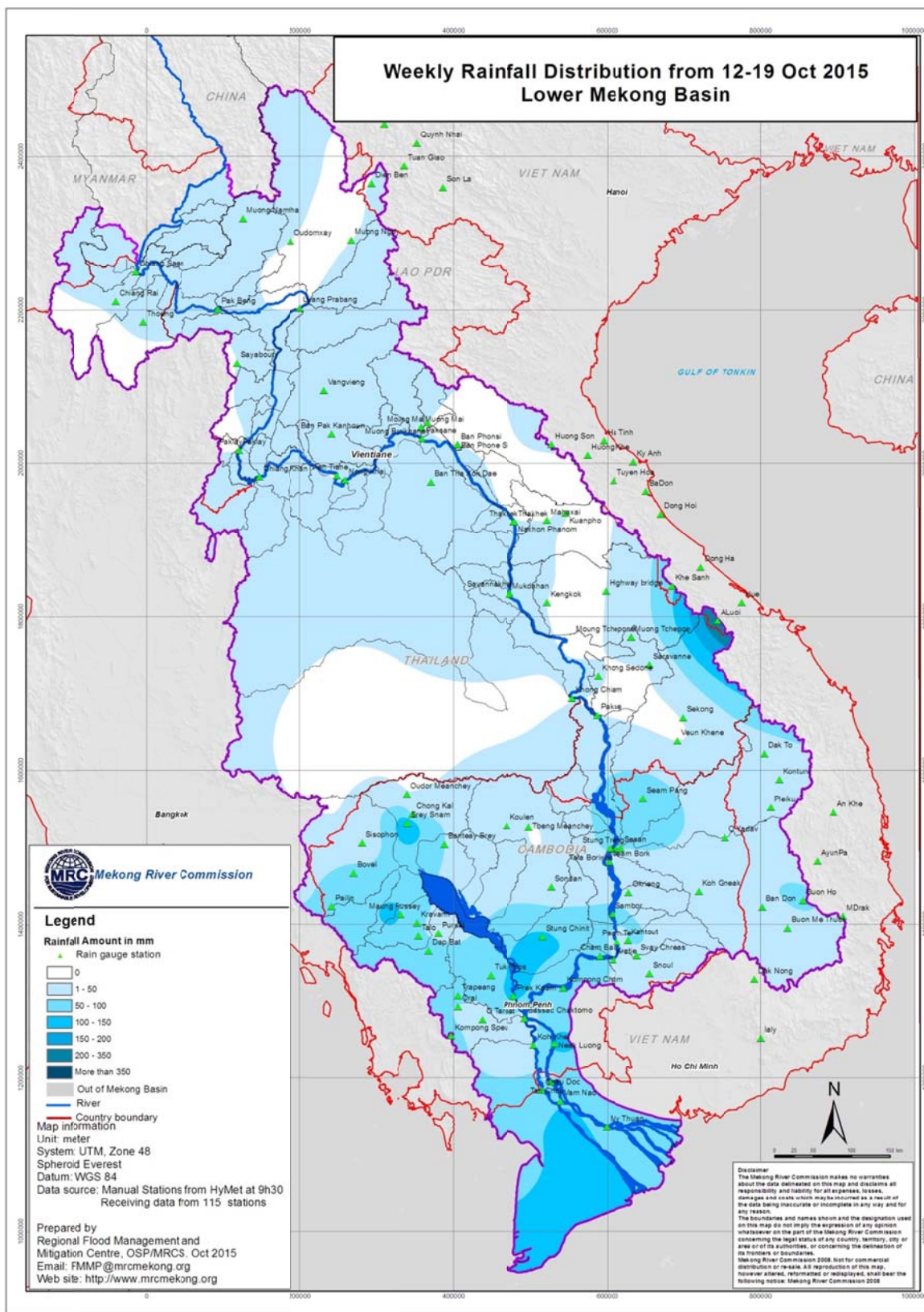
Figure 3: Weekly Rainfall Distribution over the LMB from 12 th October - 19 th October 2015
