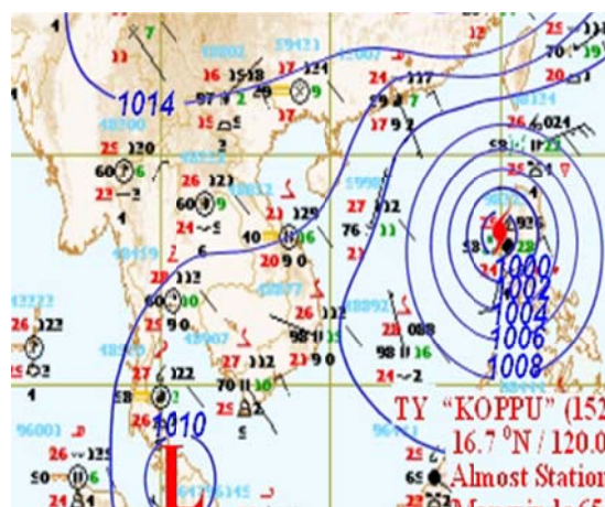
Figure 2: Weather map for 18 th October 2015
